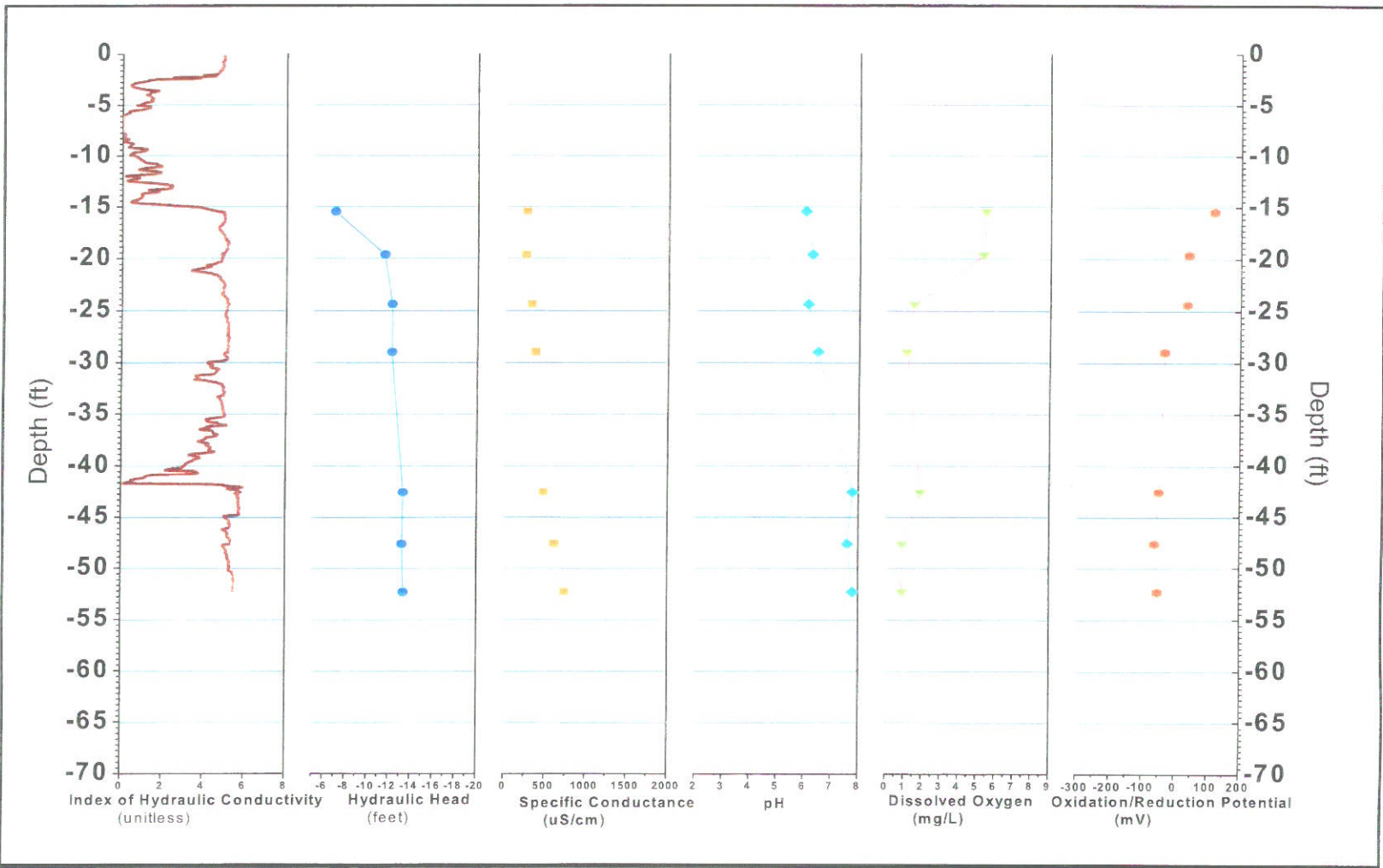
FIGURE B-234, I K RECORD AND PHYSICO-CHEMICAL PARAMETERS ERM, Wayland, Massachusetts
