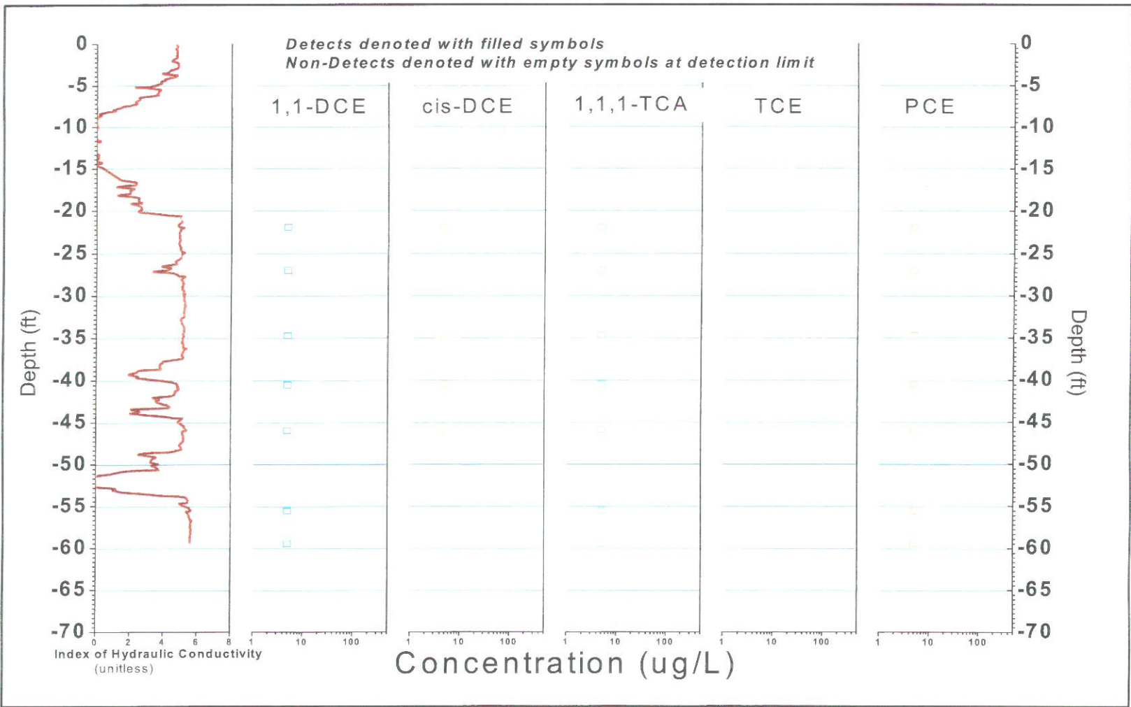
FIGURE B-235, I K RECORD AND SELECTED VOC ANALYTICAL RESULTS ERM, Wayland, Massachusetts
