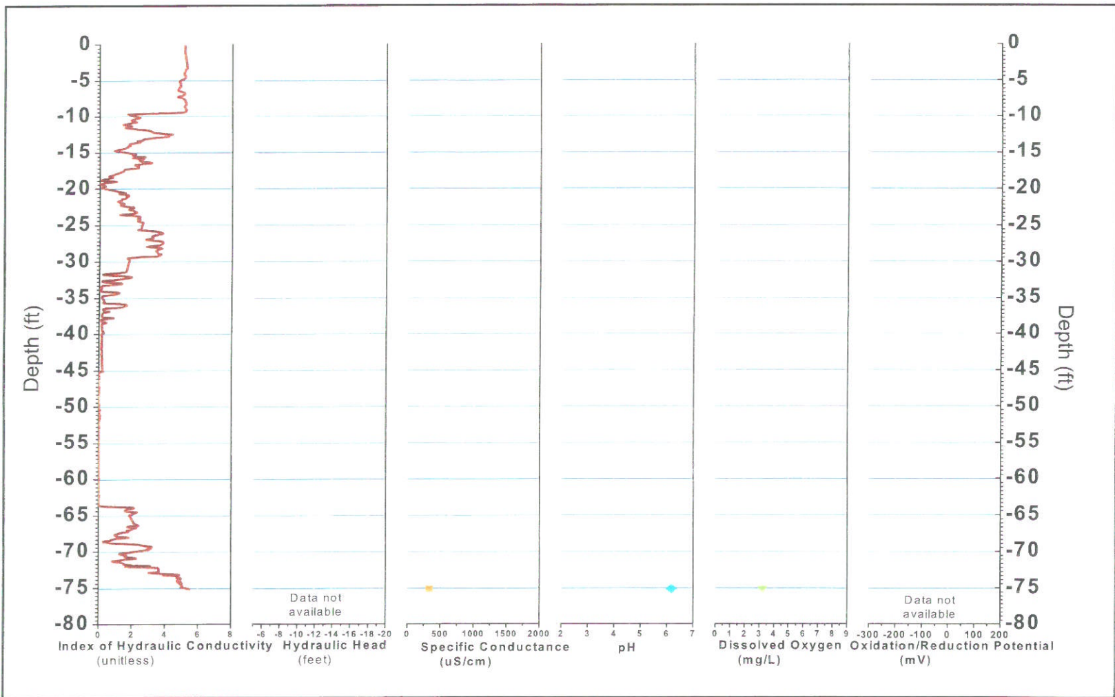
FIGURE B-232, I k RECORD AND PHYSICO-CHEMICAL PARAMETERS ERM, Wayland, Massachusetts
