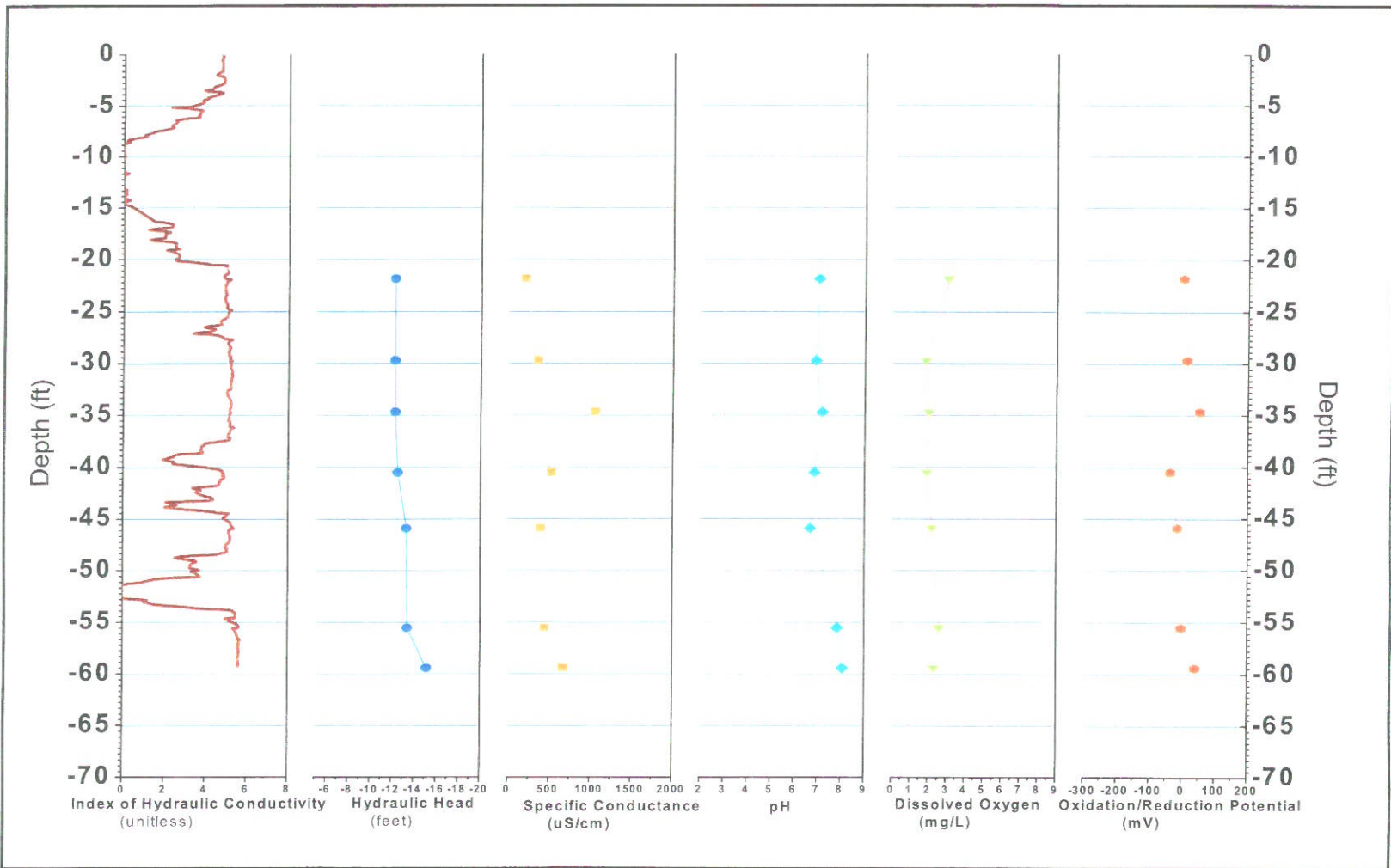
FIGURE B-235, I_K RECORD AND PHYSICO-CHEMICAL PARAMETERS ERM, Wayland, Massachusetts
