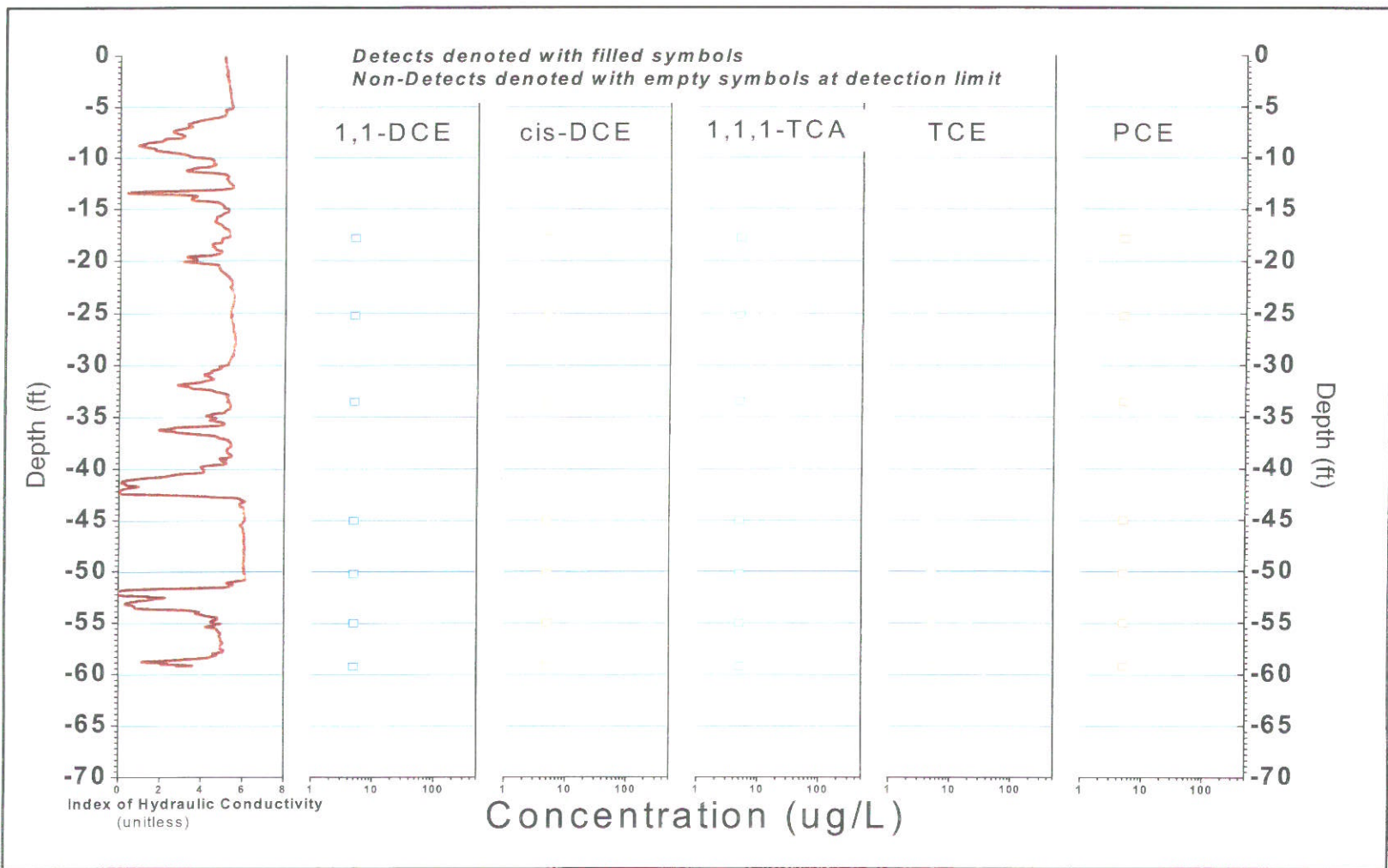
FIGURE B-233, I_K RECORD AND SELECTED VOC ANALYTICAL RESULTS ERM, Wayland, Massachusetts
