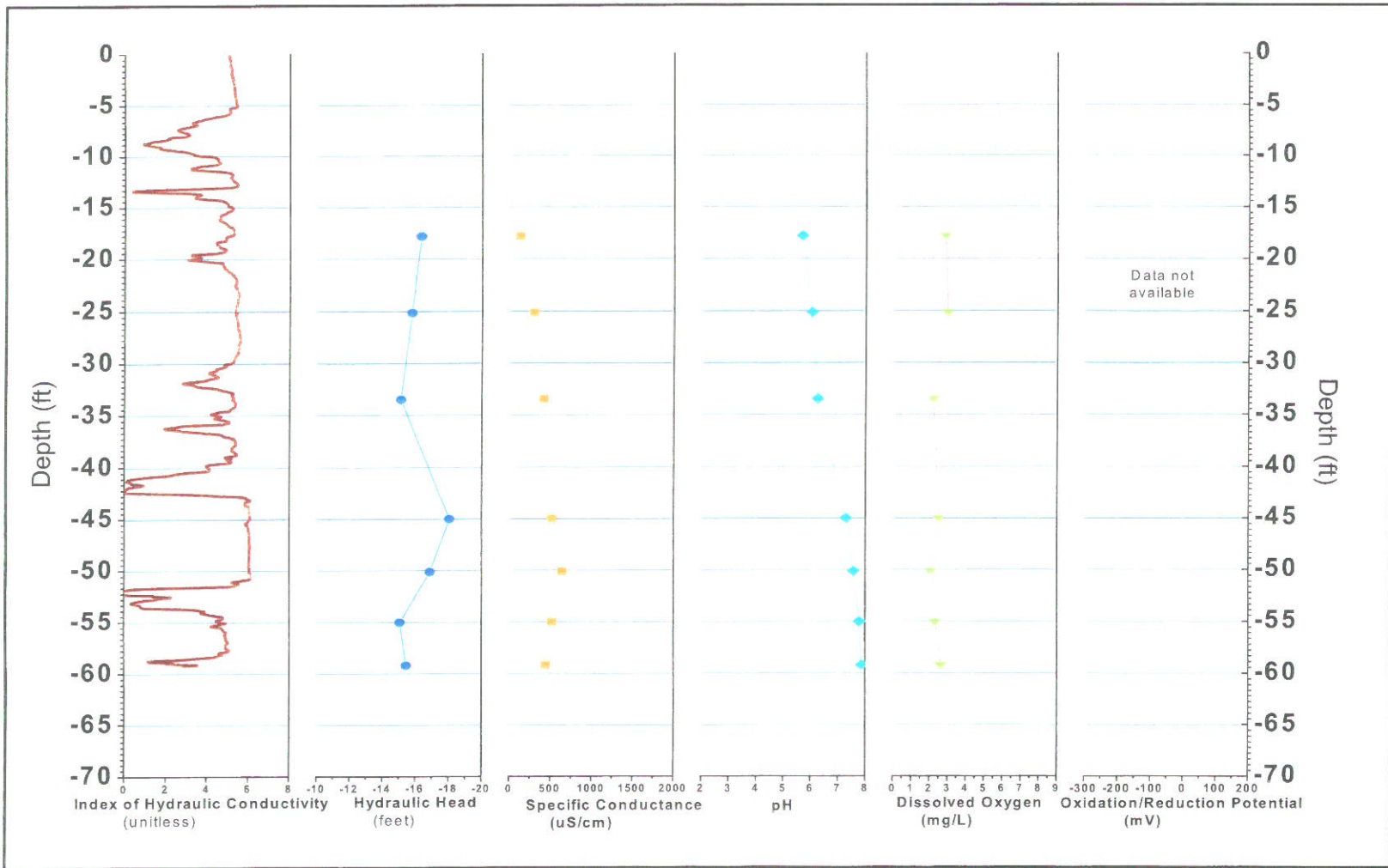
FIGURE B-233, I k RECORD AND PHYSICO-CHEMICAL PARAMETERS ERM, Wayland, Massachusetts
