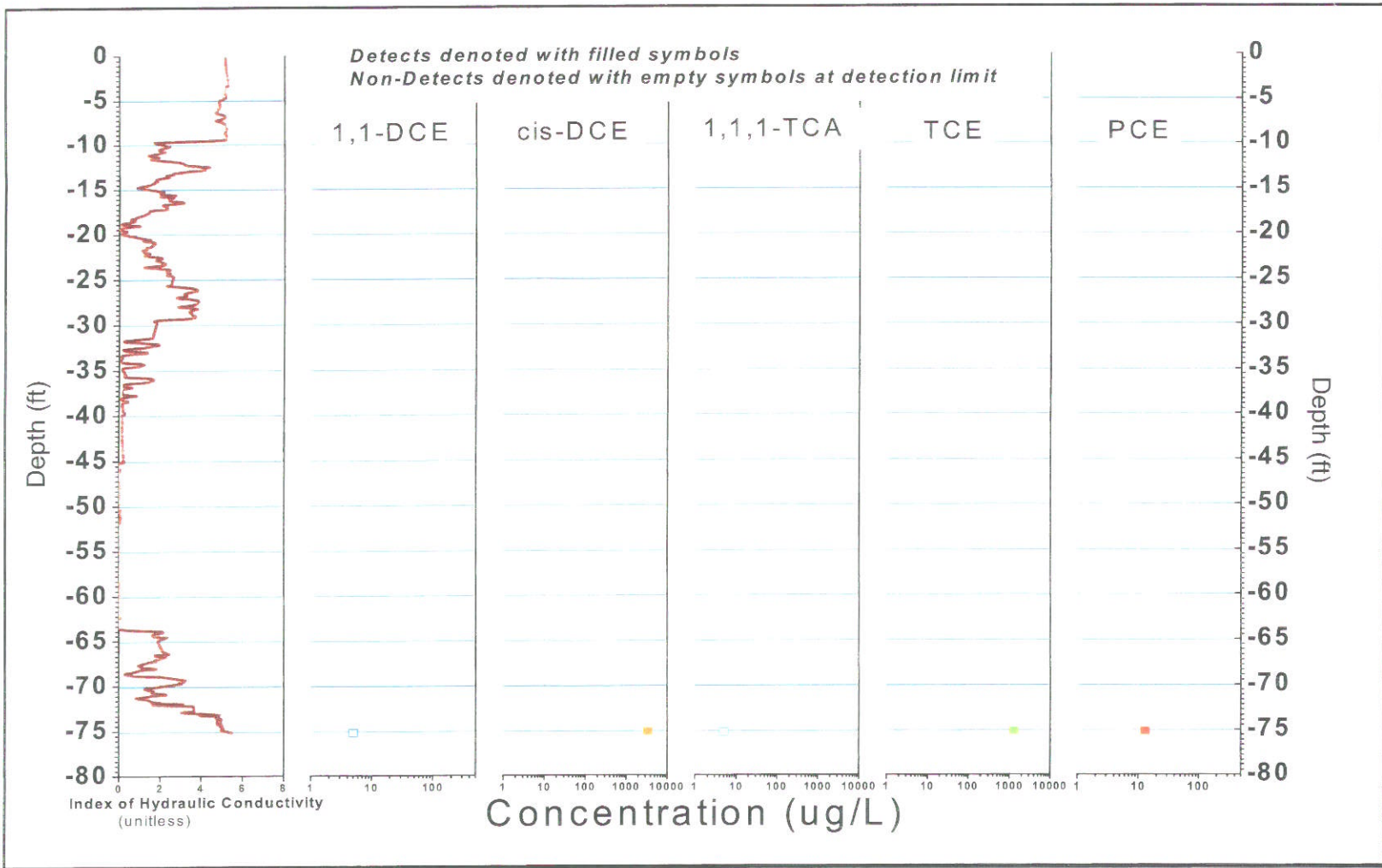
FIGURE B-232, k RECORD AND SELECTED VOC ANALYTICAL RESULTS ERM, Wayland, Massachusetts
