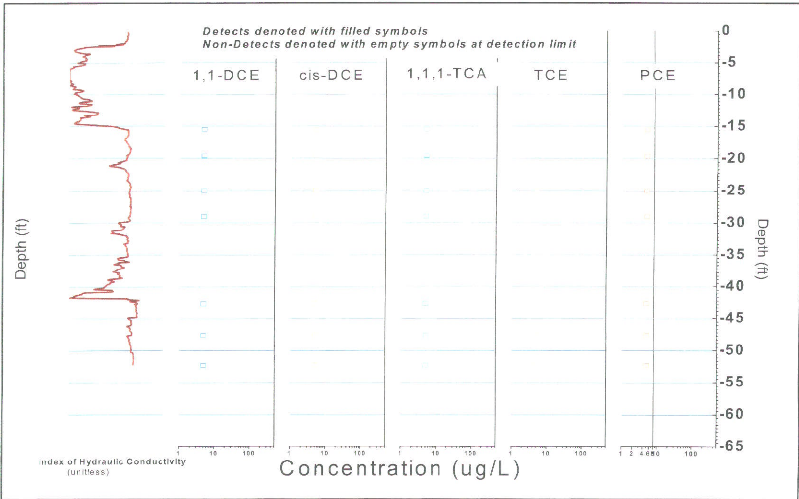
FIGURE B-234, I_k RECORD AND SELECTED VOC ANALYTICAL RESULTS ERM, Wayland, Massachusetts
